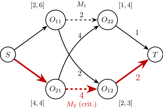
(a) G^-(\sigma) , C_{\max}^- = 6
