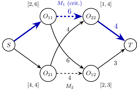
(b) G^+(\sigma) , C_{\max}^+ = 10
