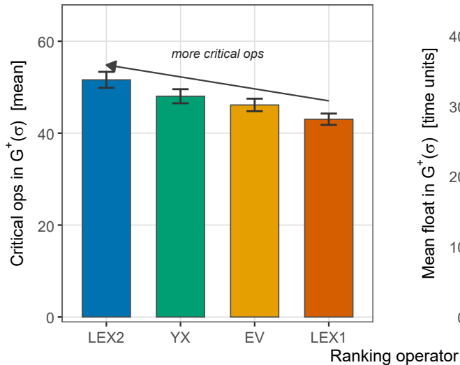
(a) G^+ critical-path saturation
