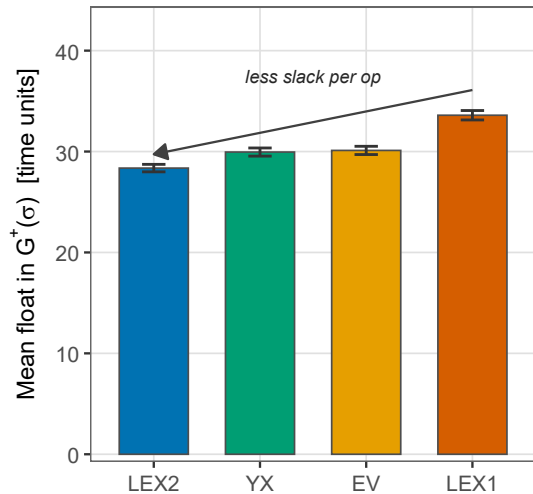
(b) Per-operation slack in G^+(\sigma)
