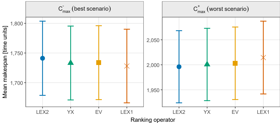
Phase A — Decomposition: C_{\max}^- (best) vs C_{\max}^+ (worst) by operator
