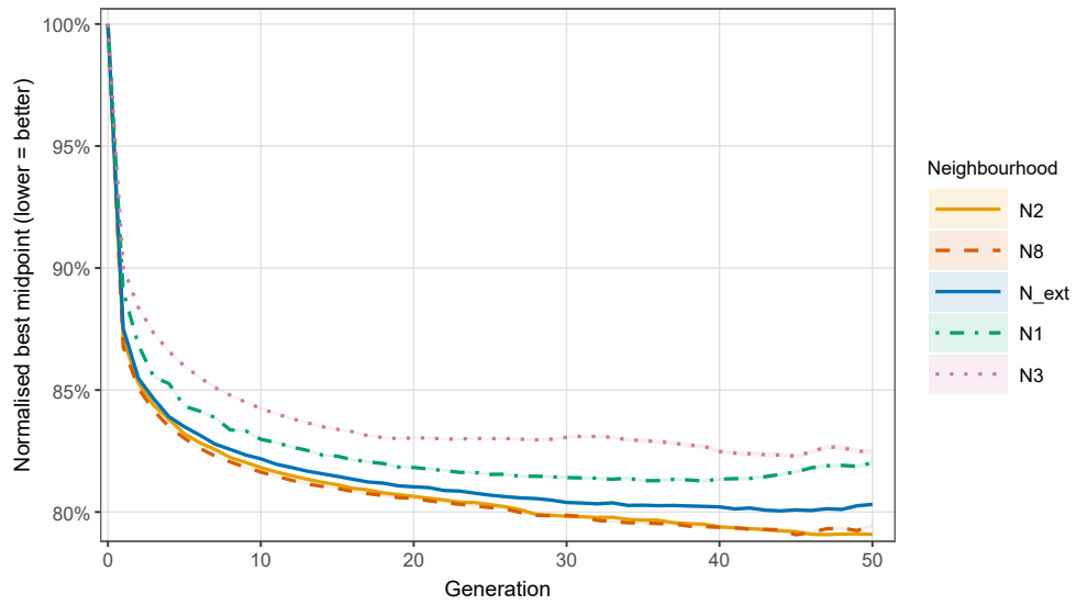
Figure 5: Per-generation normalised best-midpoint profiles, by neighbourhood (Phase B, irace-tuned tabu search; mean over 82 \text{ instances} \times 30 \text{ runs} per neighbourhood). The shaded ribbons represent \pm 1 standard error. All five neighbourhoods converge quickly (within \sim 10 generations) and then plateau; N_2 and N_8 reach the lowest final values (0.793 and 0.799), consistent with their joint statistical lead in Table 5.
