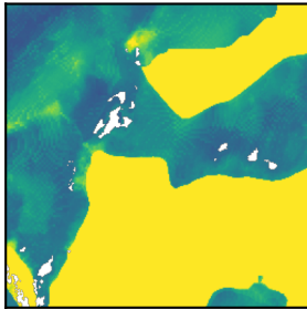
Random Forest
