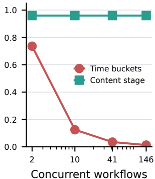
B Timing fails with overlap
