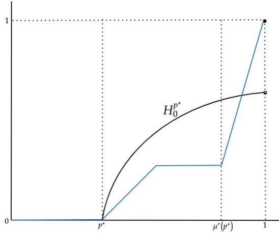
Figure 1: For uniform distribution, the optimal price p^* ( \approx 0.417 ) solves the relaxed problem and generates the distribution of buyer valuation, conditional on being recommended price p^* , represented above in blue. This distribution crosses H_0^{p^*} once and from below and hence is a mean preserving contraction of H_0^{p^*} .
