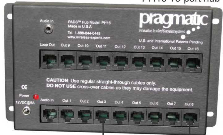
PH16 16-port hub
