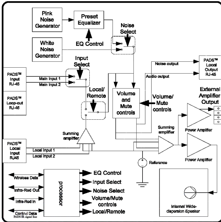
PTS-SMBGM1 Block Diagram
