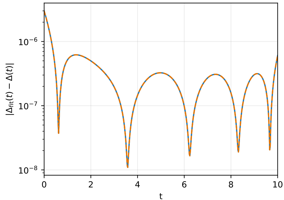
Pointwise absolute error, N=12 (7 active)
