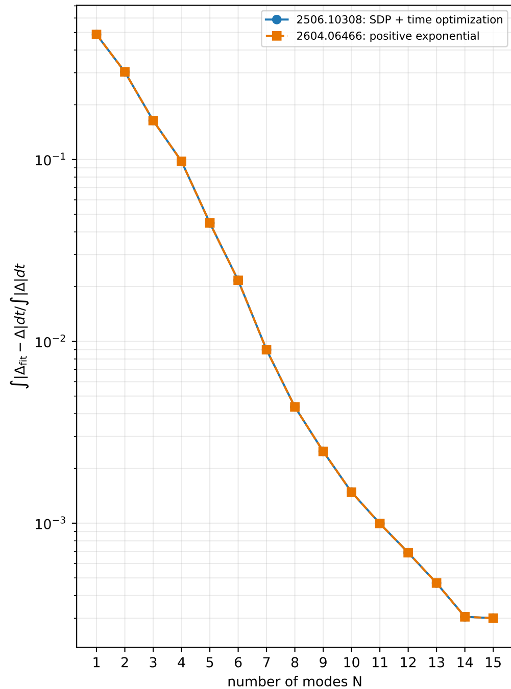
Normalized L^1 error
