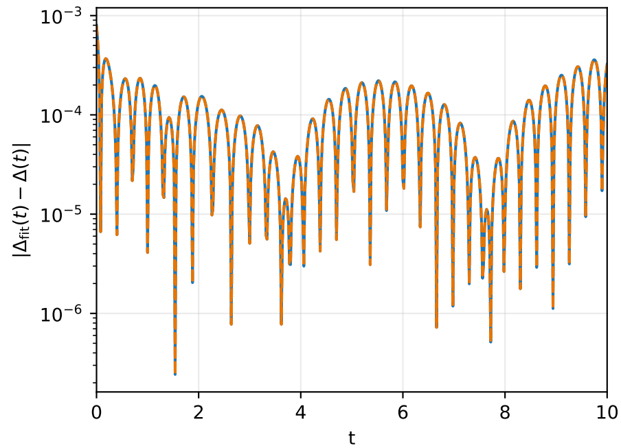
Pointwise absolute error, N=12
