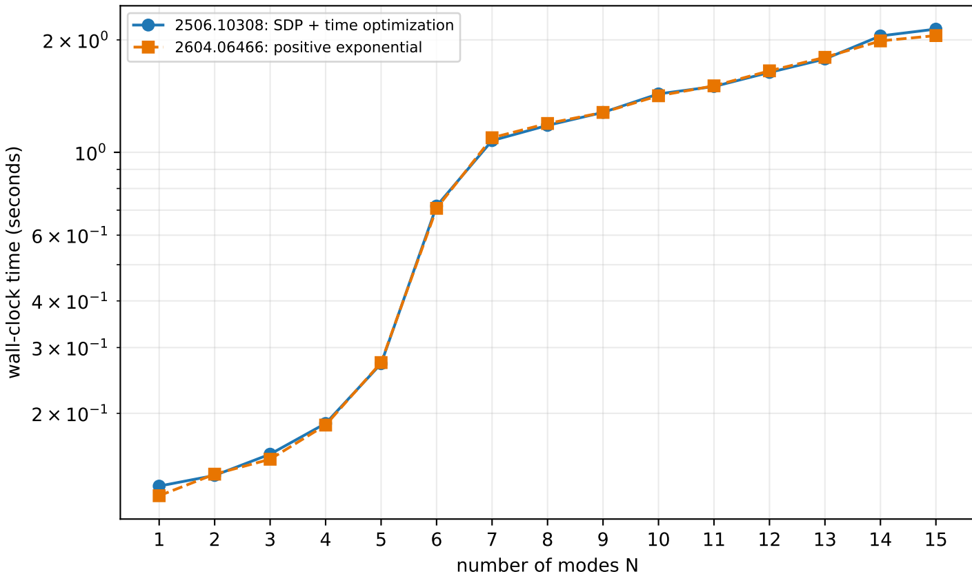
Semicircular hybridization fitting time
