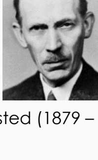
Brønsted (1879 – 1947)
