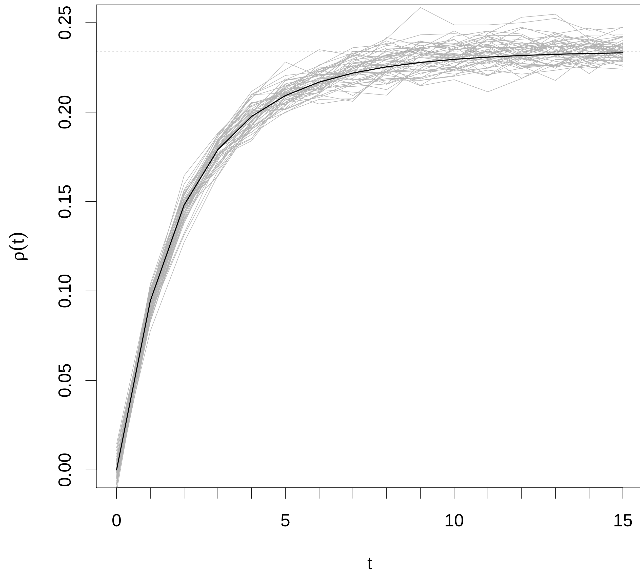
population size 25,000
