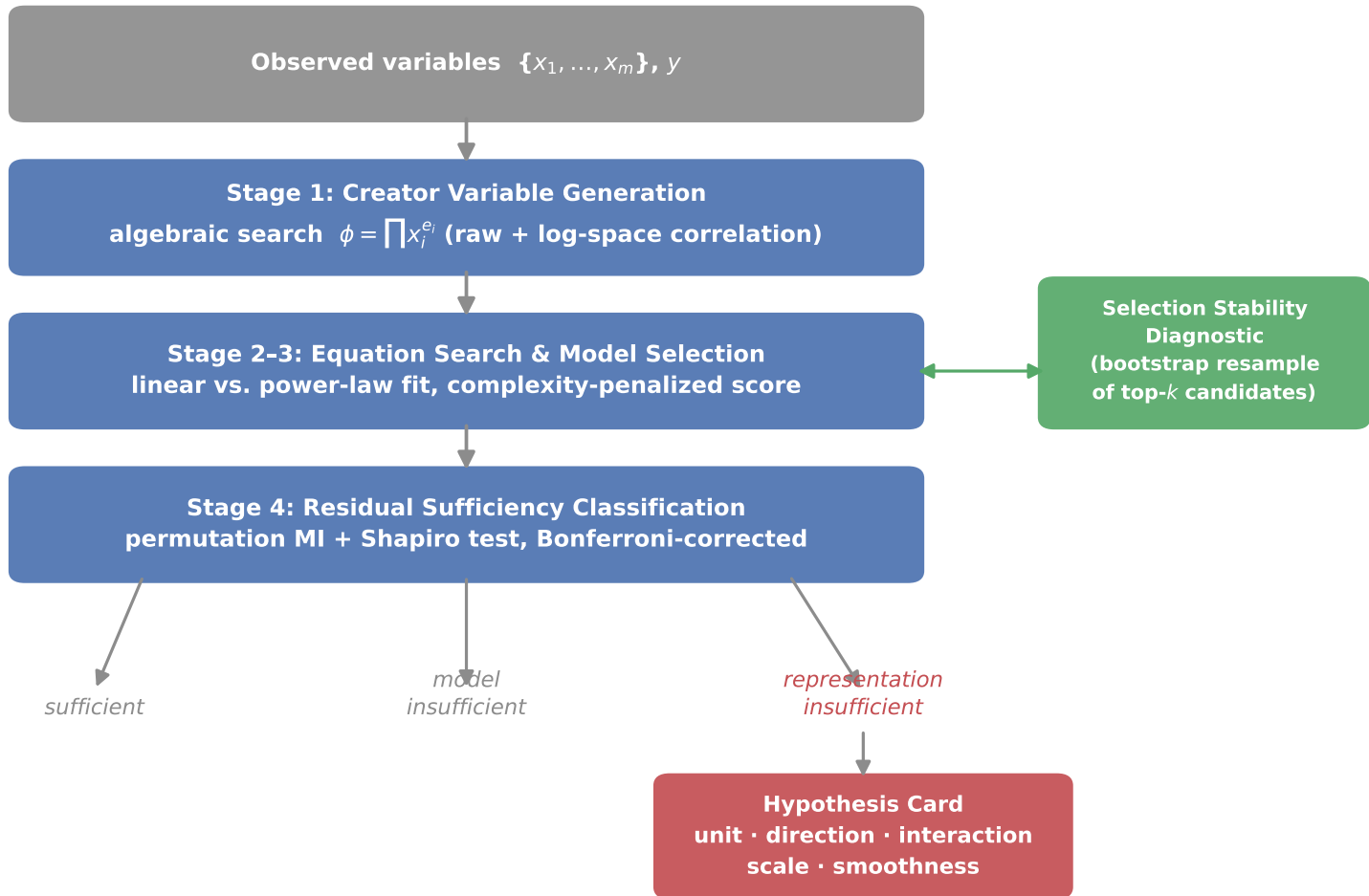
Fig. 1. CVM four-stage workflow. The selection-stability diagnostic (green) audits the Stage 2-3 model choice that all downstream inference is conditioned on.
