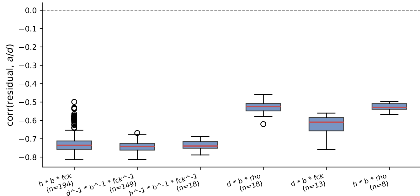
Fig. 5. WOR: \text{corr}(\text{residual}, a/d) stays negative across all 400 bootstrap resamples, regardless of which near-tied candidate wins Stage 1–3 selection
