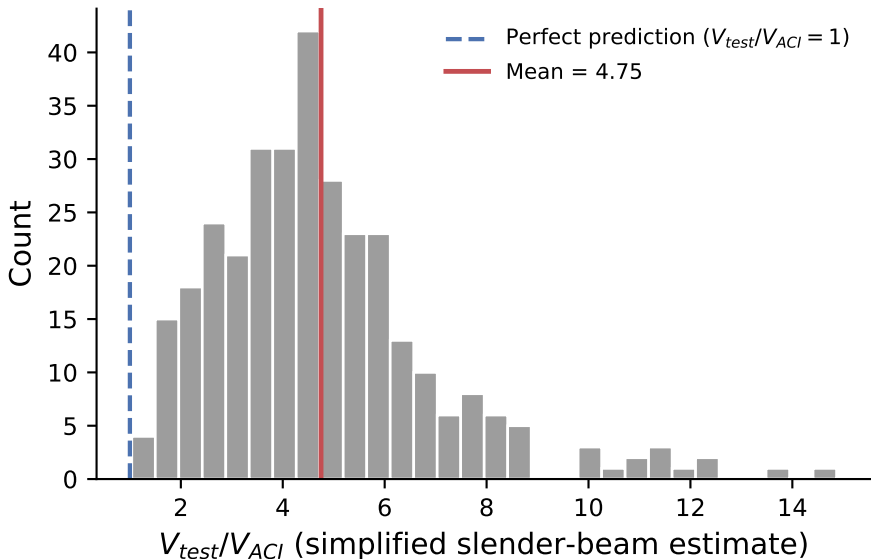
Fig. 7. ACI 318 slender-beam V_c underestimates deep-beam capacity (ACI R^2=-0.49 )
