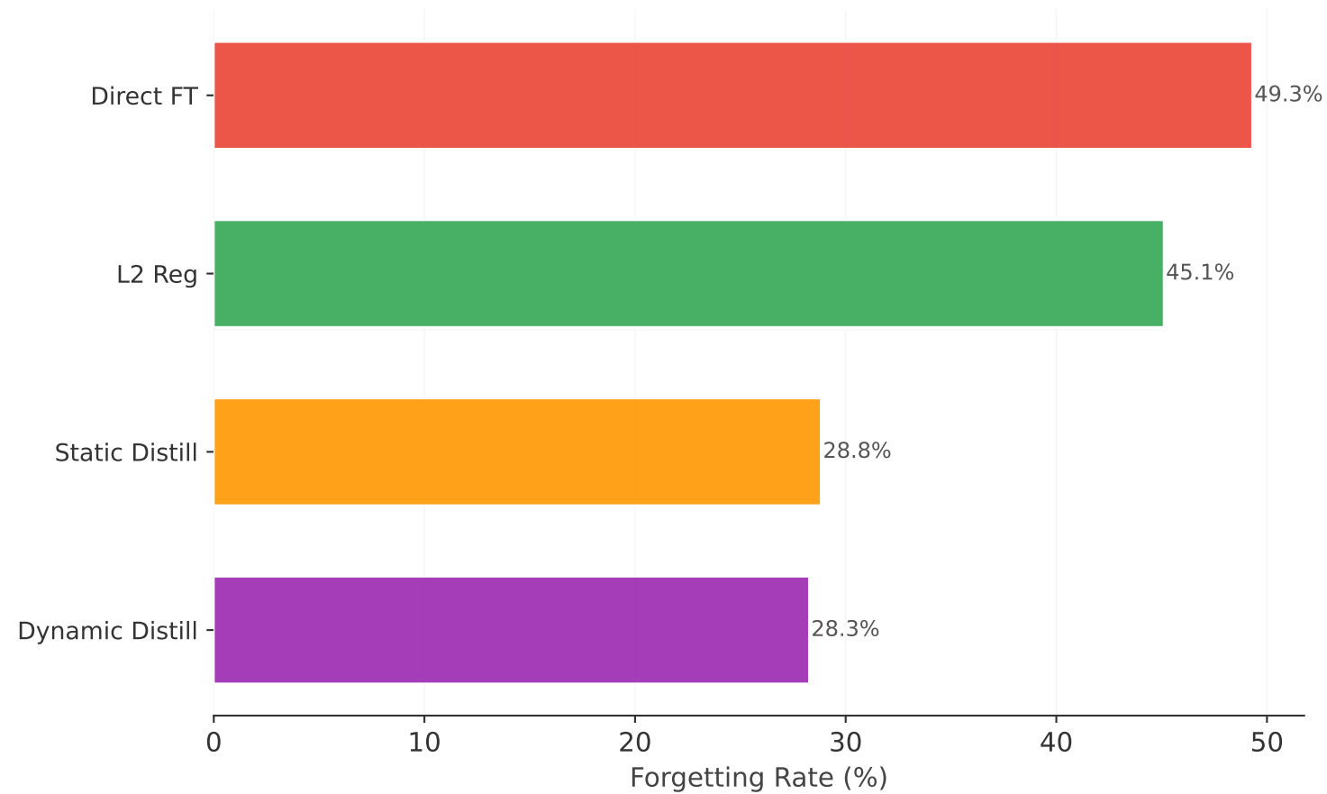
Catastrophic Forgetting
