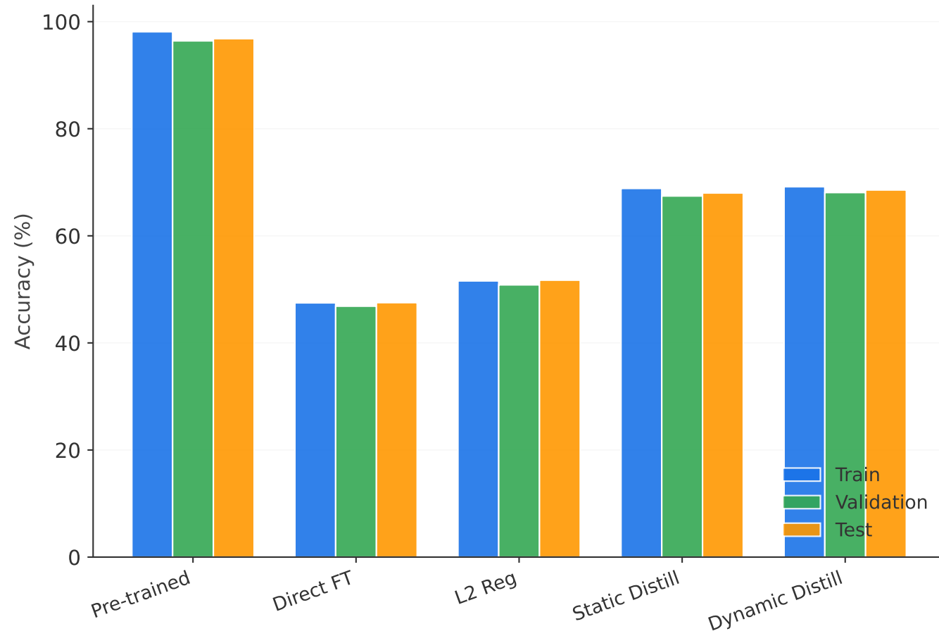
Catastrophic Forgetting
