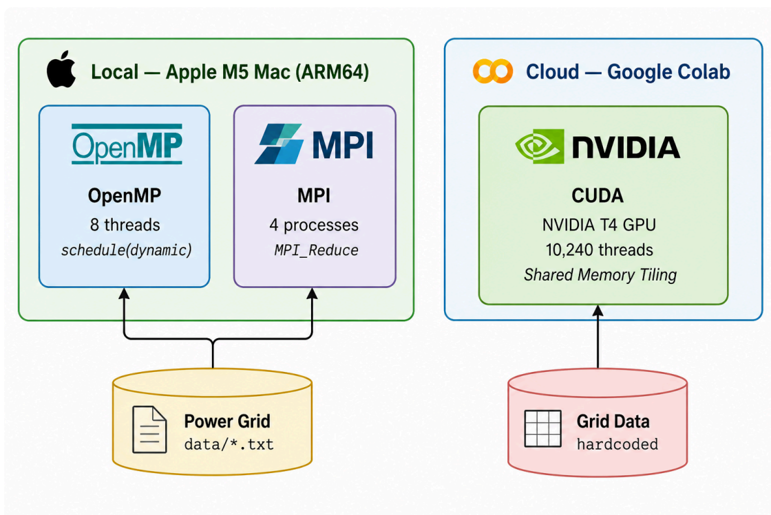
System Architecture — OpenMP and MPI run locally on Apple M5, CUDA runs on Google Colab NVIDIA T4
