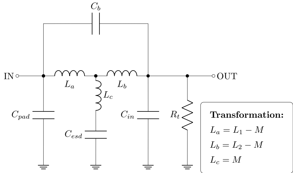
Analytical Bridged-T Network (Star Model)
