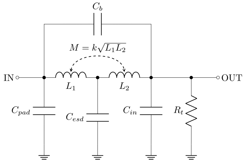
Physical T-Coil Network (Coupled Model)
