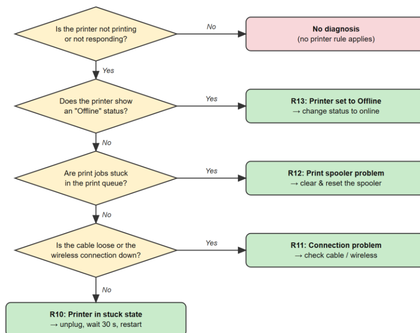
Figure 3: Example Decision Path - Printer Problems (Rules R10-R13)
