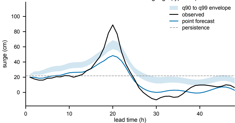
Zero-shot forecast at a held-out gauge (typhoon)
