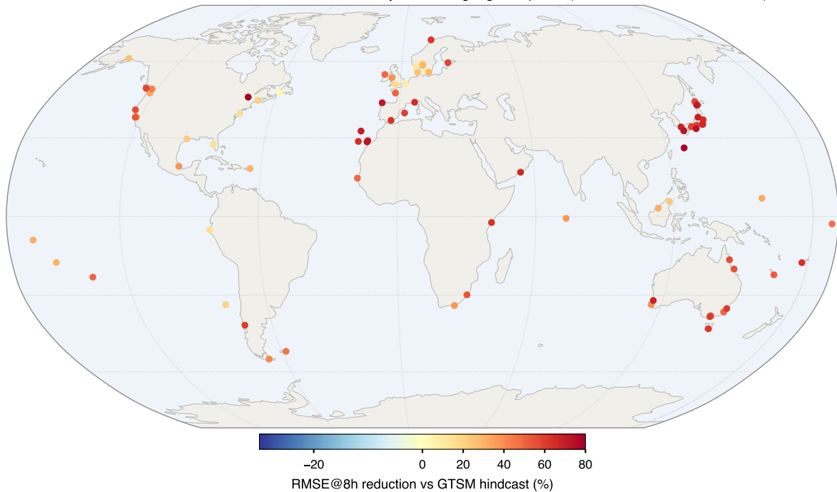
zero-shot forecast vs ERA5-forced GTSM reanalysis: 79/80 gauges improve (identical windows, 2010-2018)
