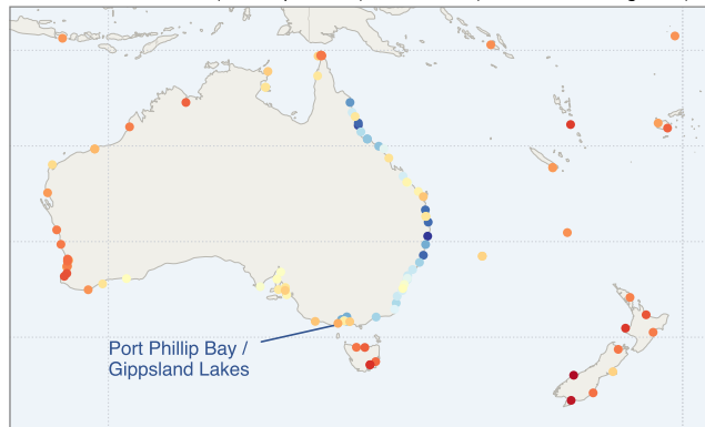
d held out: Oceania (+11% pooled (median of 3), n=111 , 38 negative)
