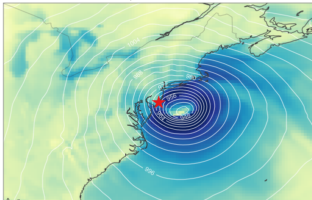
f Sandy (Oct 2012), Atlantic City GEFS +45 h, valid 2012-10-29 21 UTC
