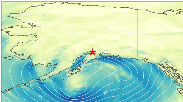
c Anchorage storm (Dec 2019), Anchorage GEFS +48 h, valid 2019-12-26 00 UTC
