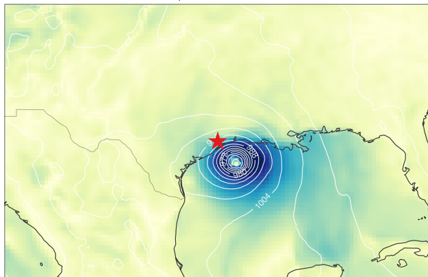
d Hurricane Ike (Sep 2008), Morgans Point GEFS +48 h, valid 2008-09-13 00 UTC
