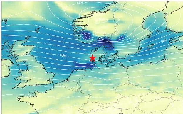
a Gudrun (Jan 2005), Esbjerg GEFS +39 h, valid 2005-01-08 15 UTC
