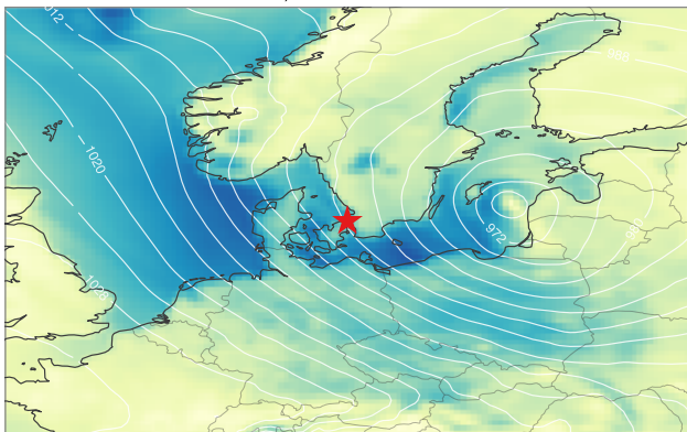
e Xavier in the Kattegat (Dec 2013), Viken GEFS +39 h, valid 2013-12-06 15 UTC
