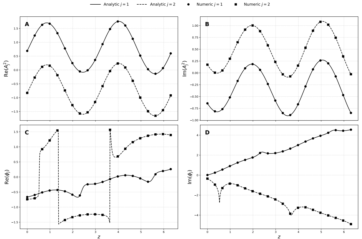
Figure 1: A real and B imaginary parts of the complex mode power A_j^2 , and C real and D imaginary parts of the complex phase variable \phi_j , using the analytic solutions in (6.9) (lines) compared against numerical integration of the original general coherent coupler system in (3.1) (symbols).
