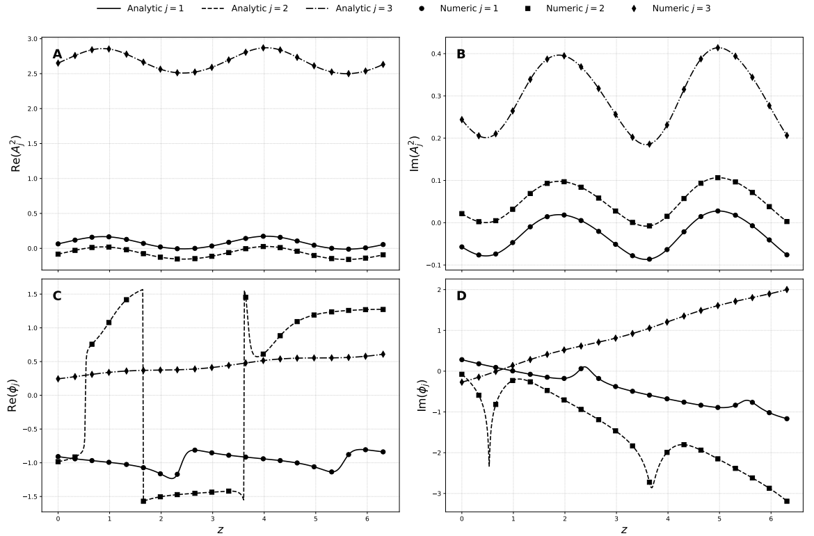
Figure 3: A real and B imaginary parts of the complex mode power A_j^2 , and C real and D imaginary parts of the complex phase variable \phi_j , using the analytic solutions in (7.26) (lines) compared against numerical integration of the three-mode degenerate FWM system in (7.18) (symbols).
