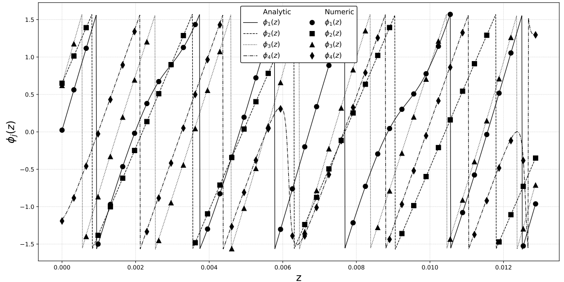
Figure 4: Phase \phi_j of physical field amplitudes: analytic solution (6.7) converted via (??) (dashed lines) compared with numerical integration (symbols).
