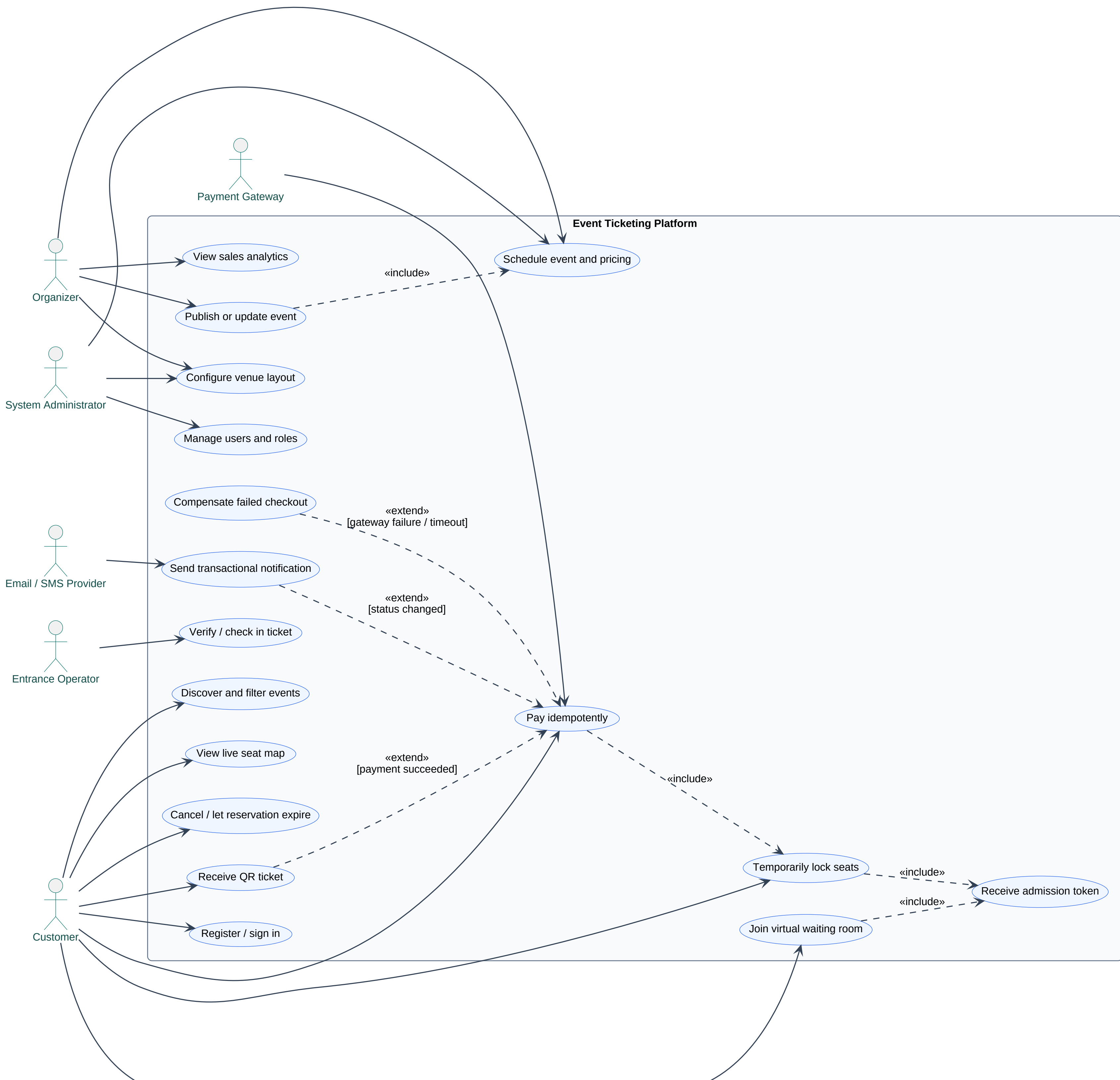
Event Ticketing Platform — Use Case Diagram
