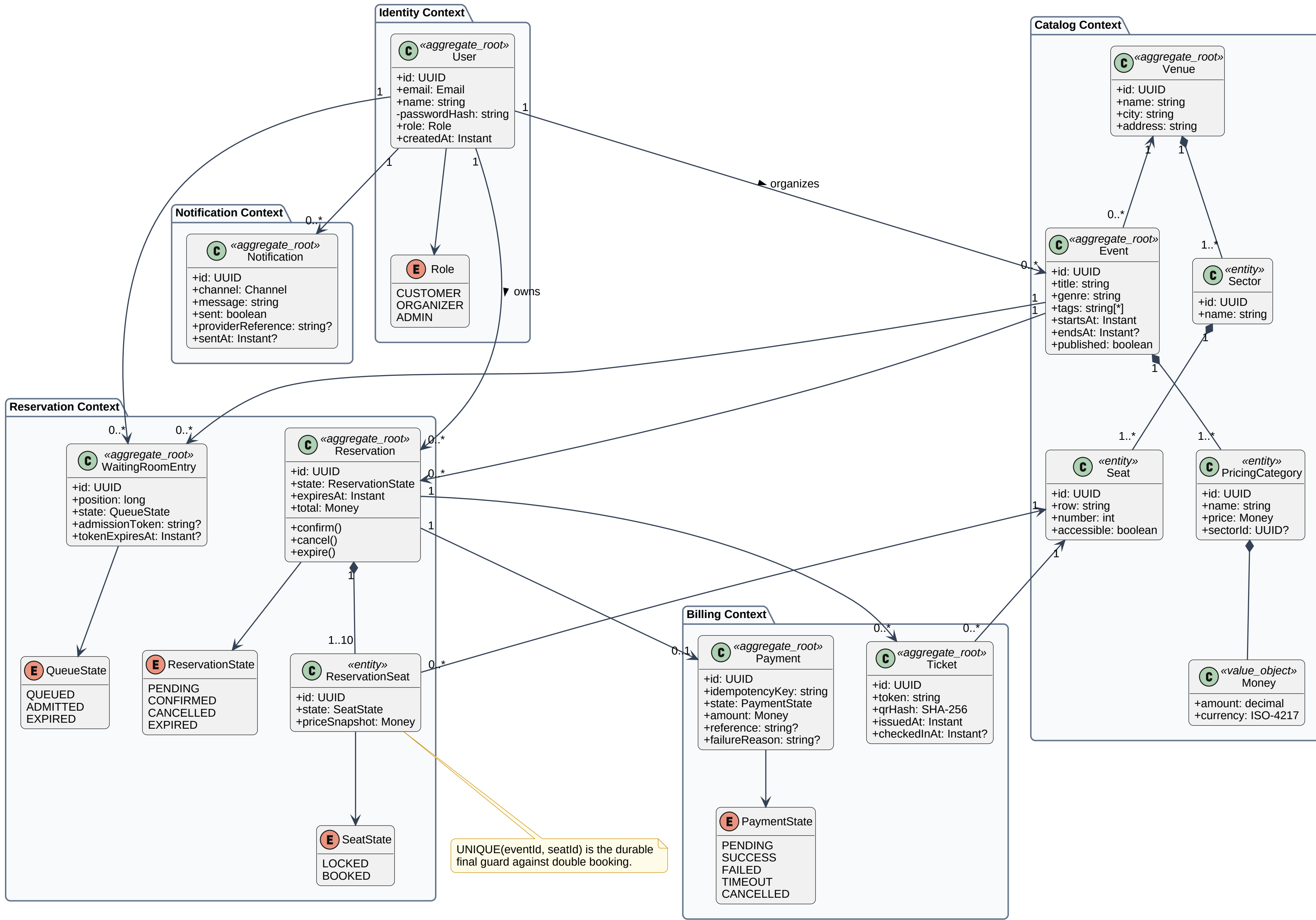
Event Ticketing Platform — Domain Class Diagram
