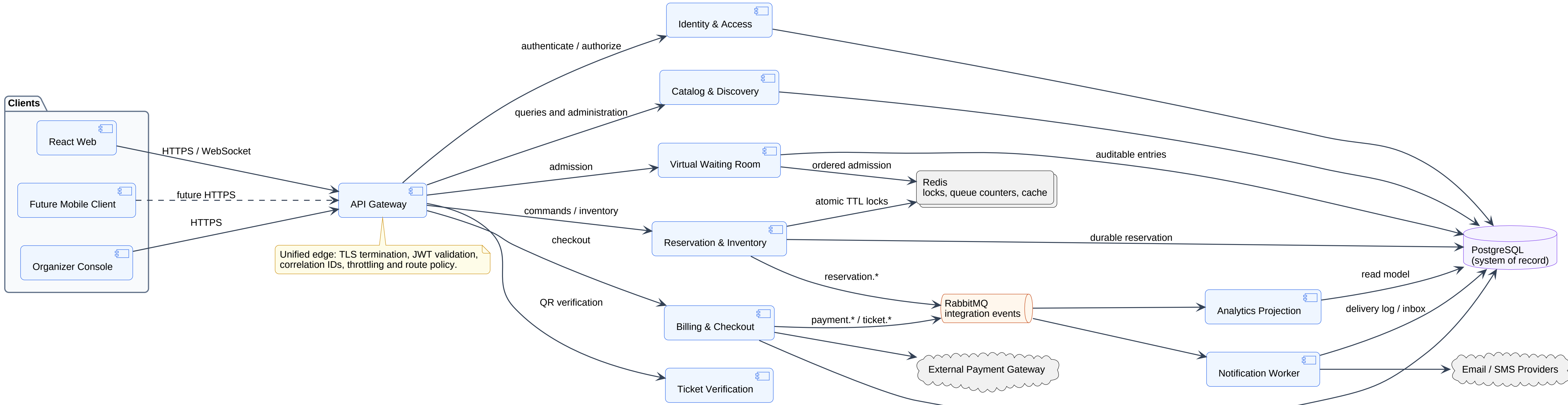
Logical Component Diagram — Decoupled Bounded Contexts
