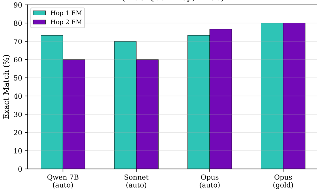
Per-Hop Extraction Accuracy by Model Scale (MuSiQue 2-hop, n=30)
