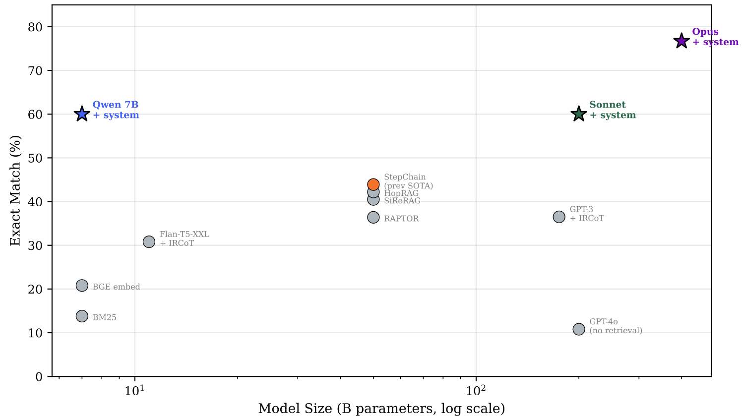
MuSiQue 2-hop: Model Size vs Accuracy (Stars = ours)
