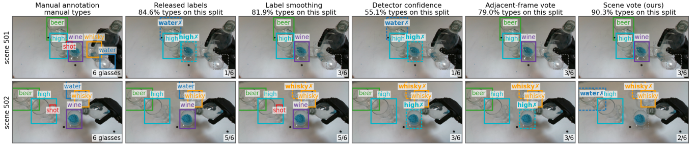
Fig. 3. The five training-label arms on OOD test frames, accelerator A seed 1337, from the frozen predictions behind Table 2. Row 1 is chosen without looking at our arm, as the frame where the released labels mistype most; row 2 is declared our worst frame on the split. Boxes are drawn at the manual location, matched by the rule of Section 3.1, and coloured by the predicted type: solid if right, dashed with a cross if wrong, grey dotted if the arm localises nothing there. Panel counts are correctly typed boxes; headings carry each arm's type accuracy over the split.
