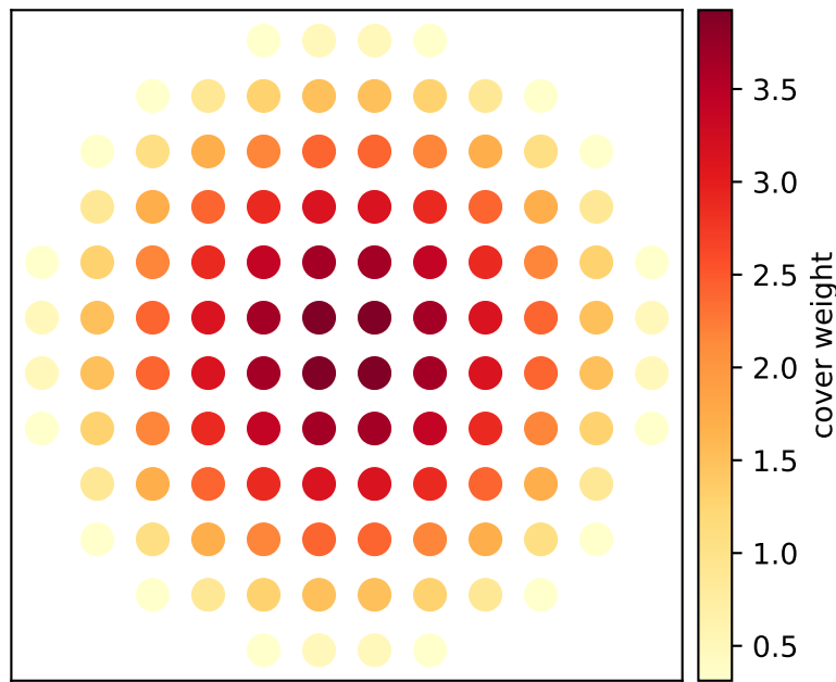
K12 sampled support
