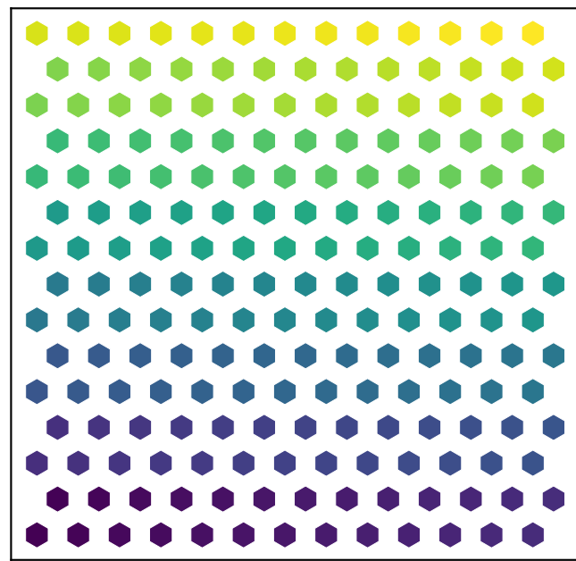
Hex token centers ( 14 \times 14 = 196 )
