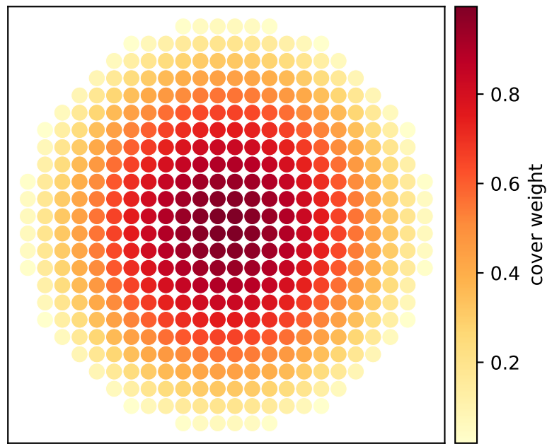
K24 sampled support
