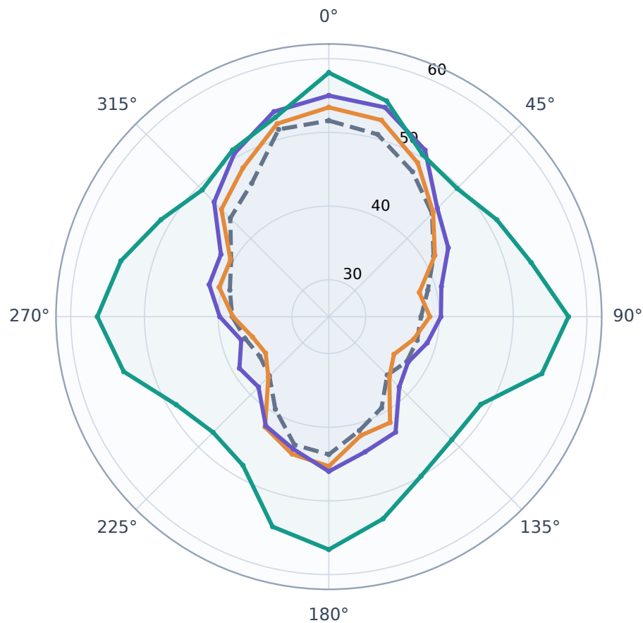
Classification accuracy by rotation
