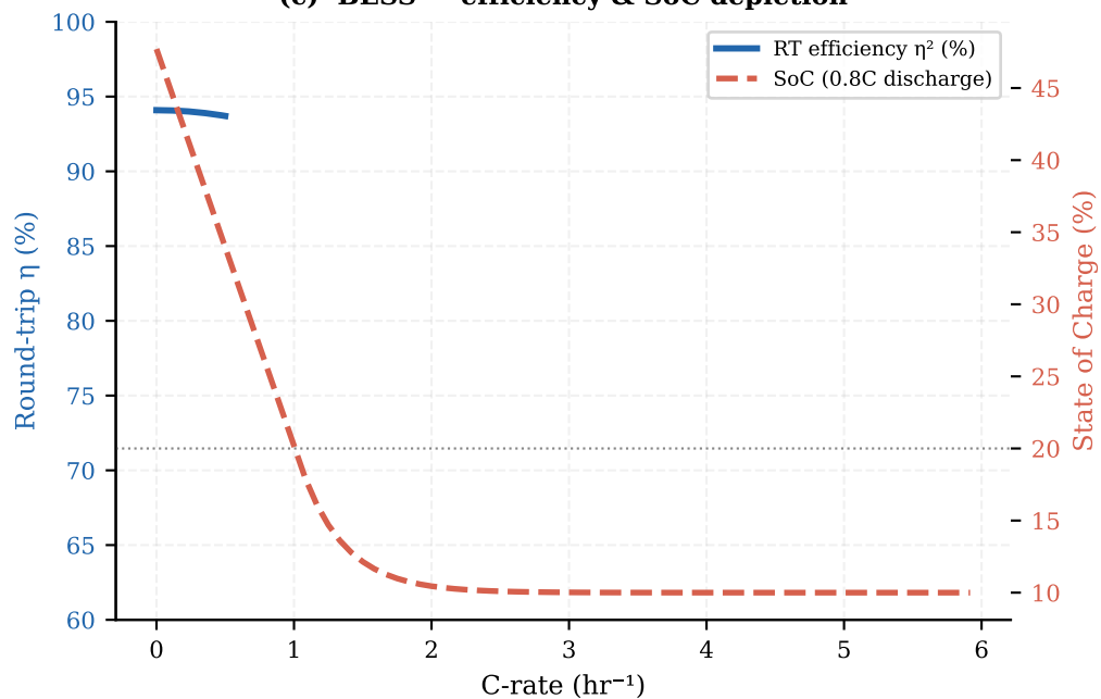
(c) BESS — efficiency & SoC depletion
