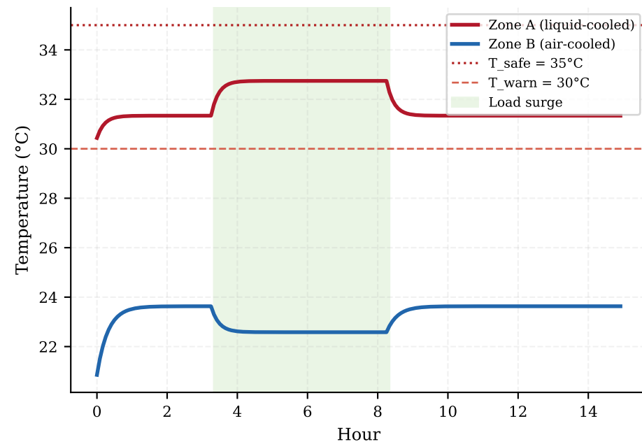
(b) ThermalTwin — step response
