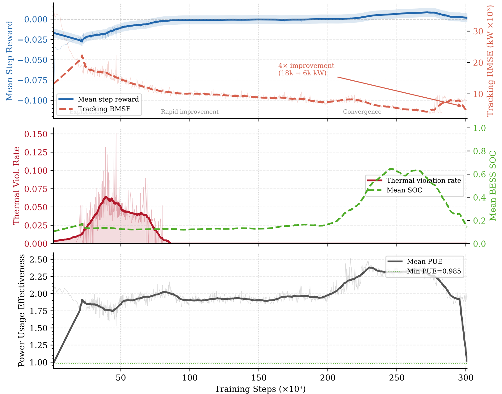
PPO Training on C2GFastEnv — default scenario, seed 42, 300k steps
