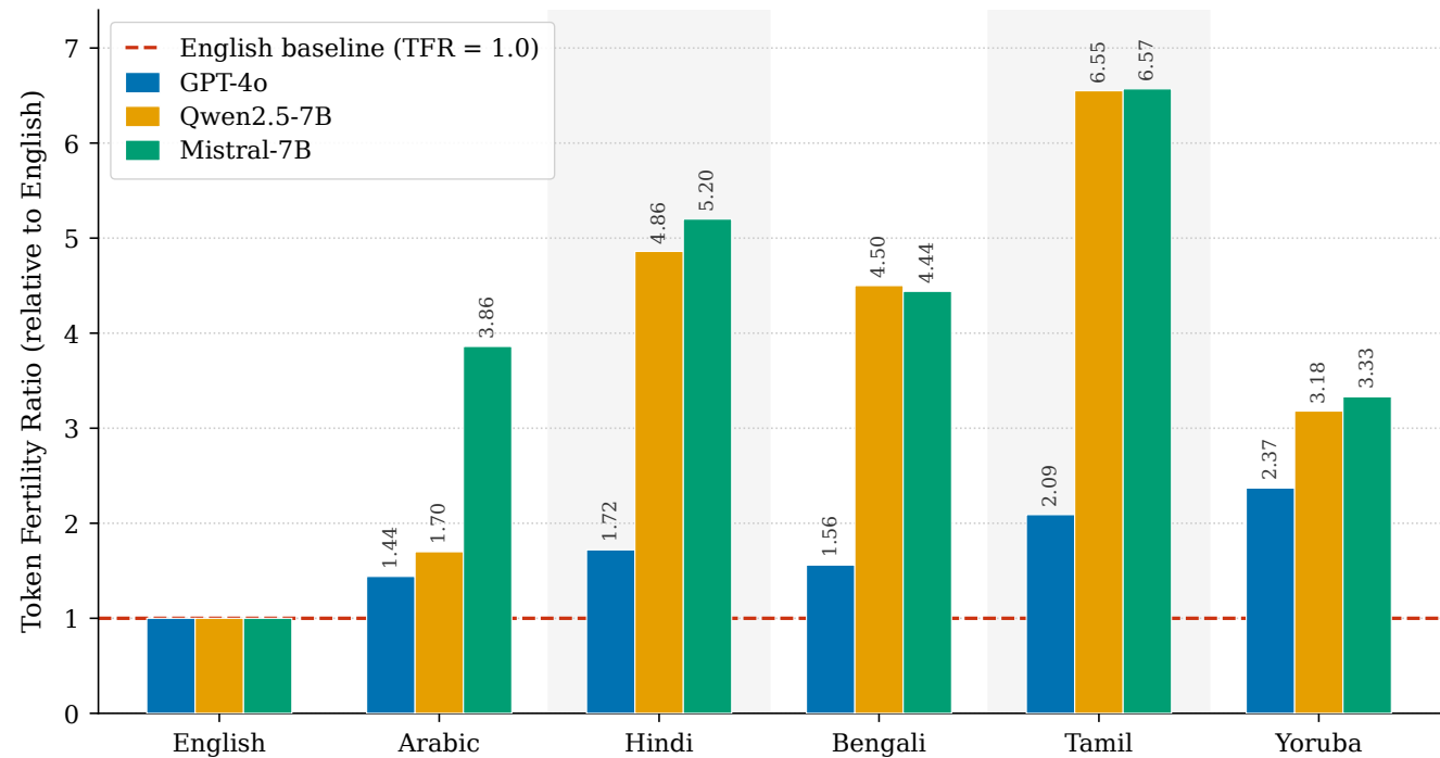
Token Fertility Ratio by Language and Tokenizer (TEA Benchmark, n = 120 )
