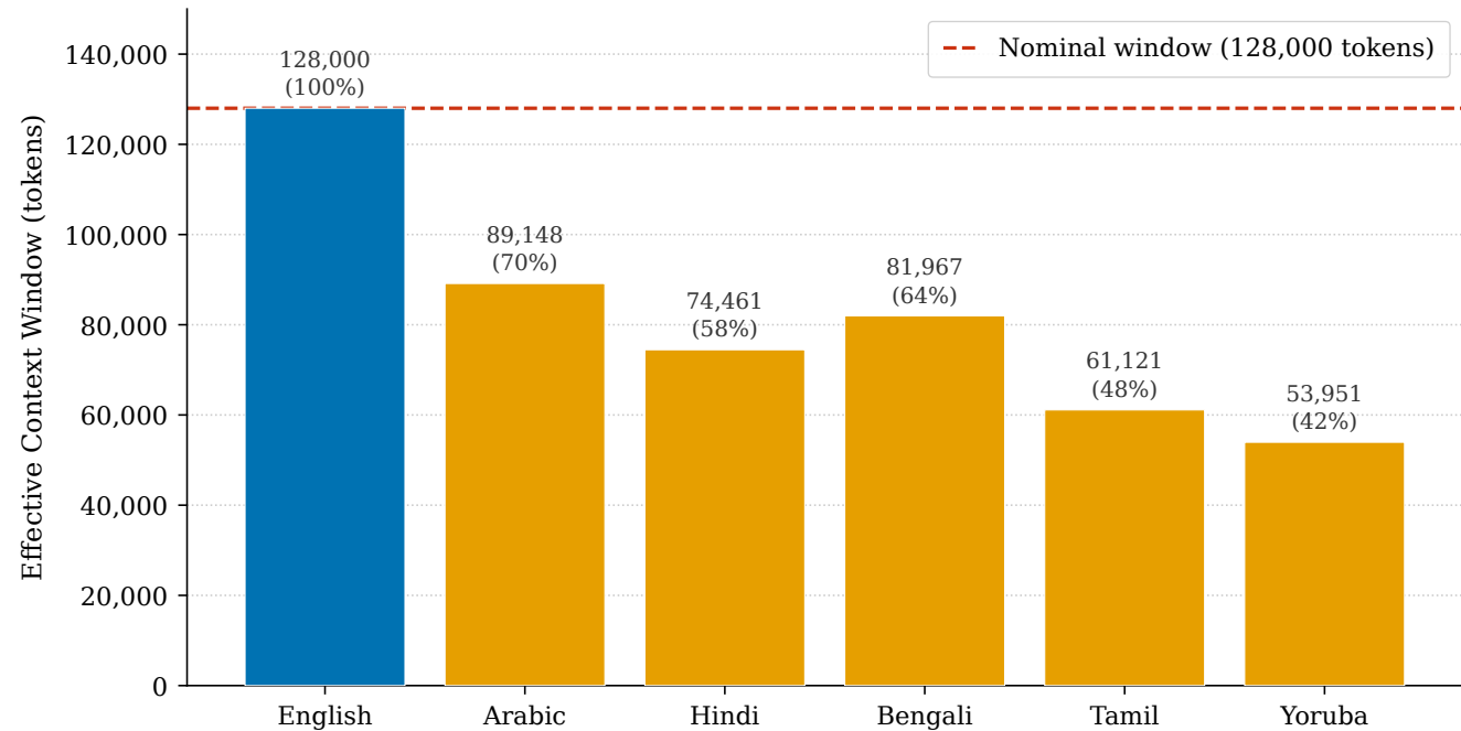
Effective Context Window Under GPT-4o Tokenization (TEA Benchmark, nominal = 128k)
