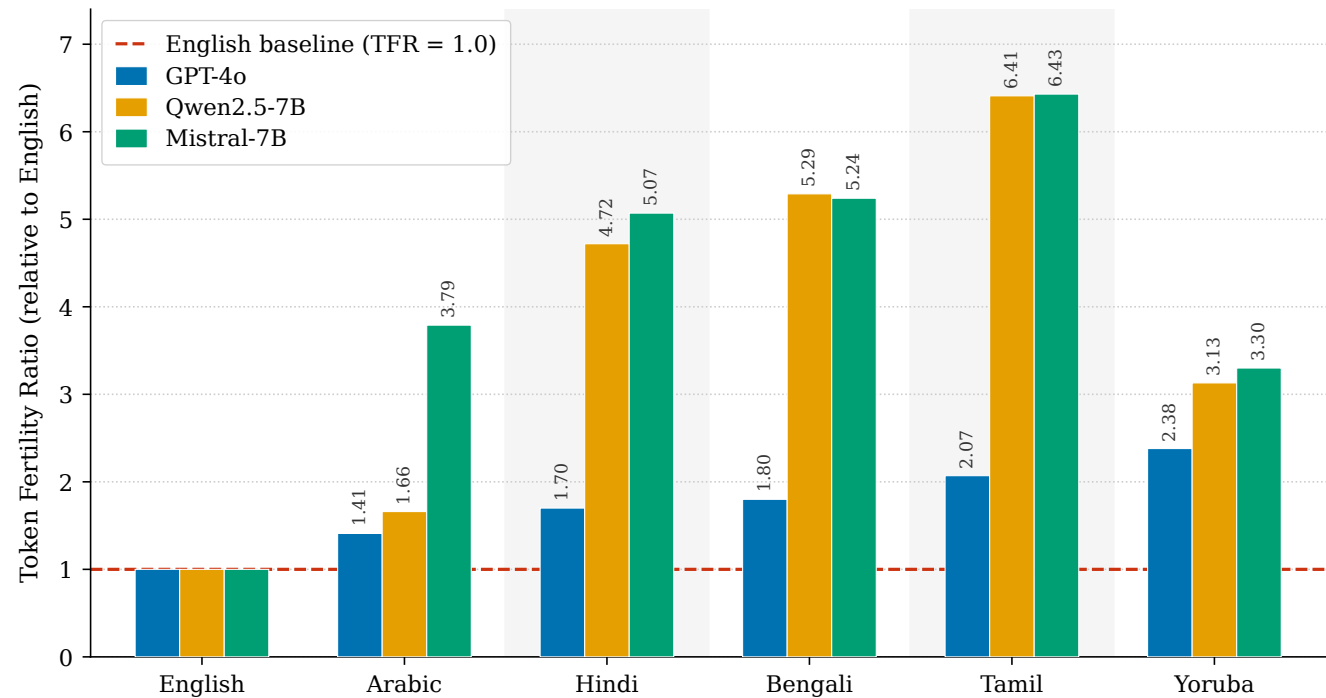
Token Fertility Ratio by Language and Tokenizer (TEA Benchmark, n = 70 )
