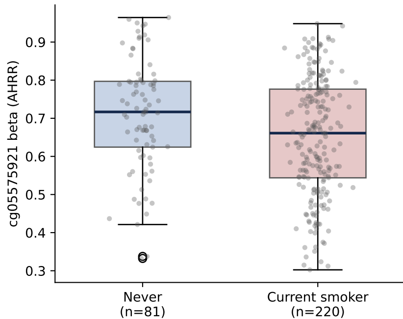
A The control R07 could not power now holds: p = 0.0056
