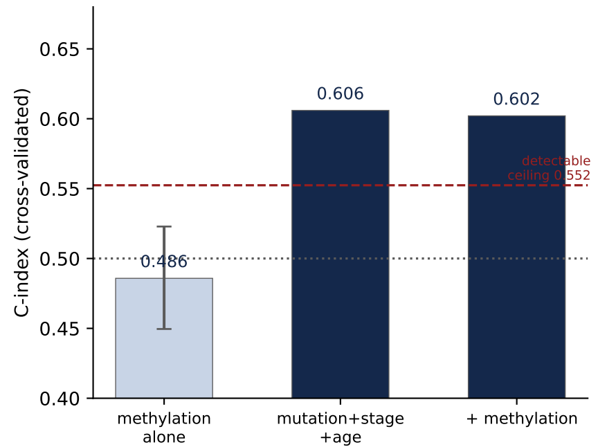
C Q3: methylation adds nothing LR p = 0.85
