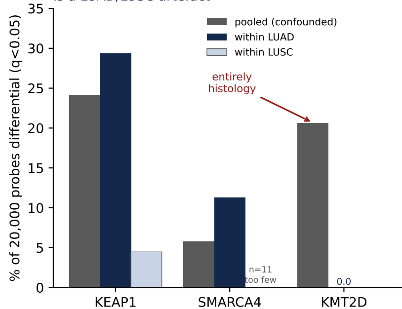
B Q1 corrected: KMT2D's phenotype is a LUAD/LUSC artefact
