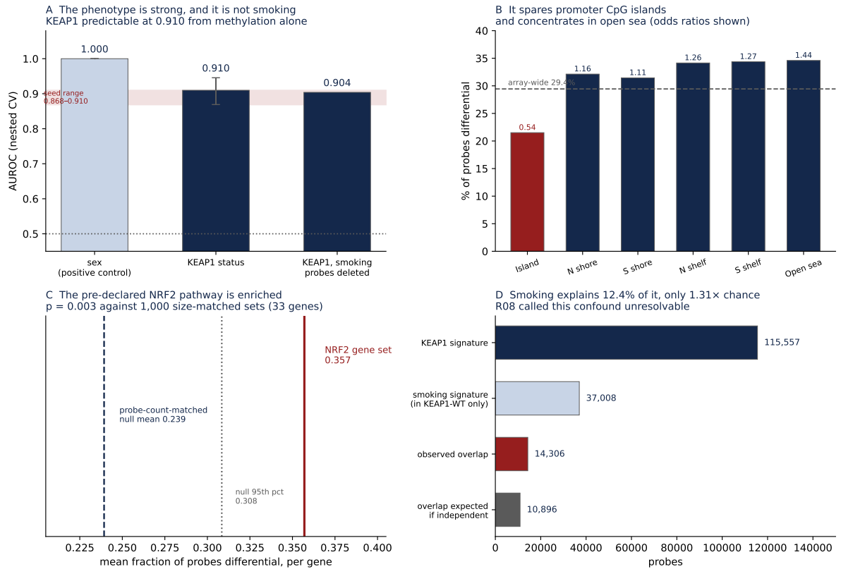
A Classifier performance, with the sex control and the smoking-deleted variant; shaded band is the 5-seed range. B Differential probes by CpG island context, odds ratios above each bar; red marks depletion. C The NRF2 gene set against 1,000 probe-count-matched random sets. D The overlap with smoking, against what chance alone would give.
