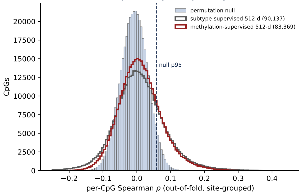
A Supervising on methylation does not help genome-wide matched dimensionality, folds, ridge — only the target differs
