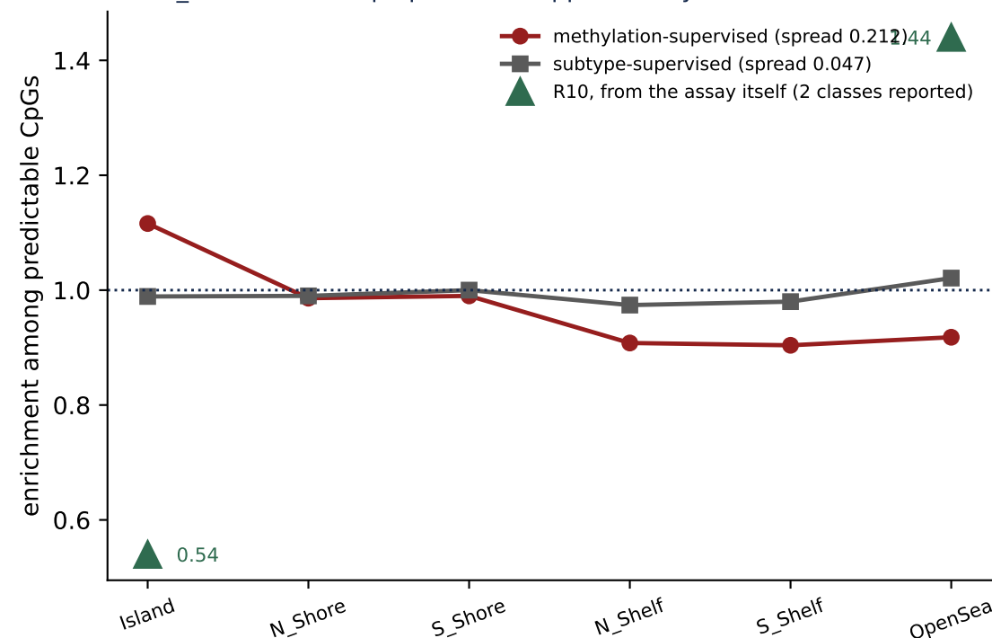
D Neither embedding recovers the assay's structure and A_meth's mild slope points the opposite way to R10
