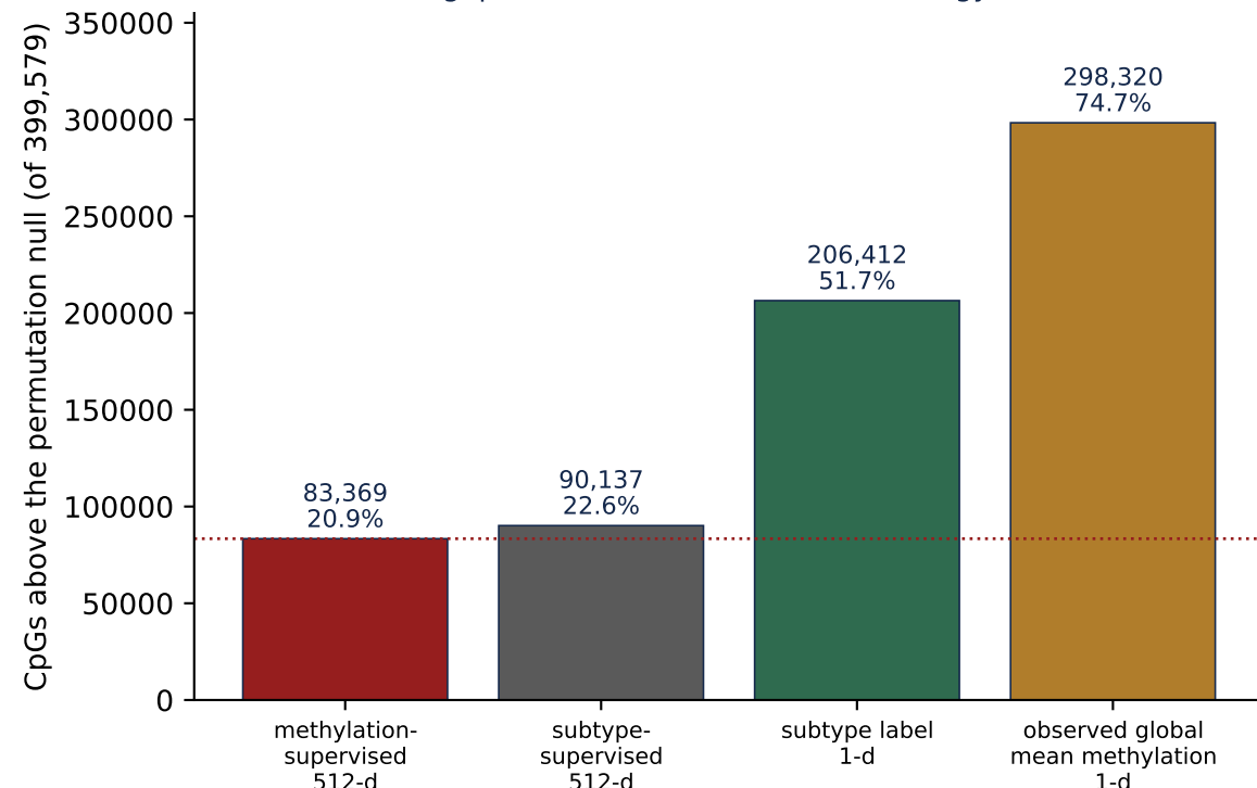
B Both embeddings lose to a single scalar the 512-d vs 1-d gap is a variance effect, not a biology one
