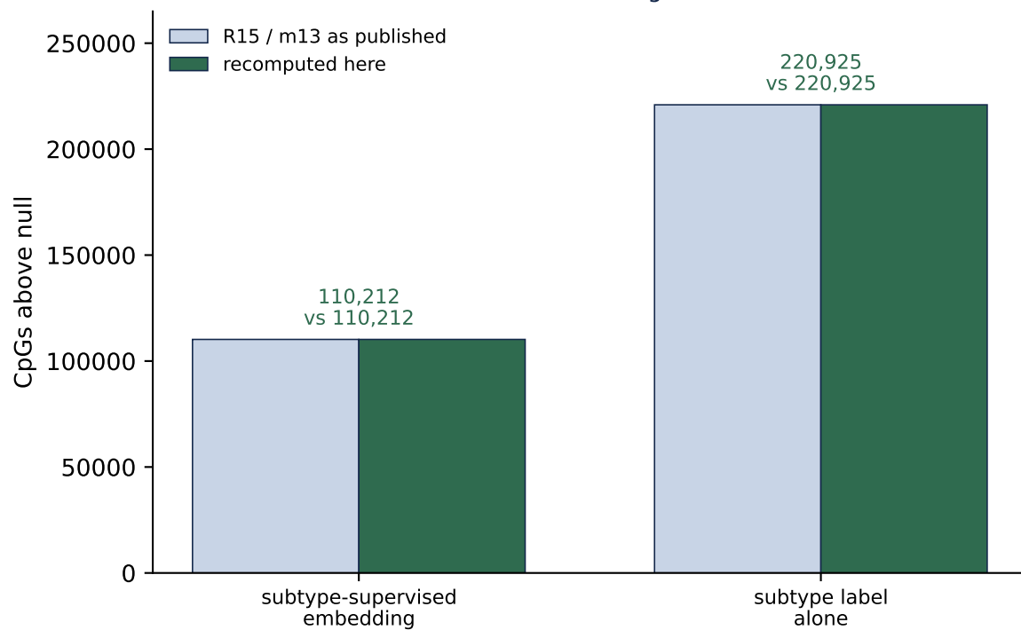
C The reimplementations reproduces R15 to the unit so the new arm's null result is not a coding difference
