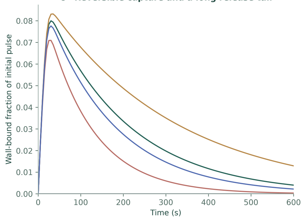
C Reversible capture and a long release tail
