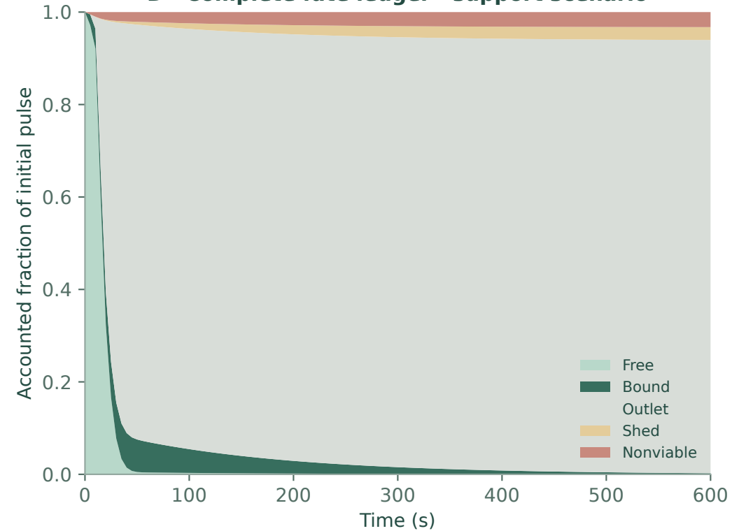
D Complete fate ledger · support scenario
