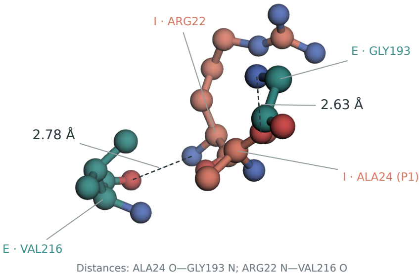
b Reactive-site contacts: selected residues
