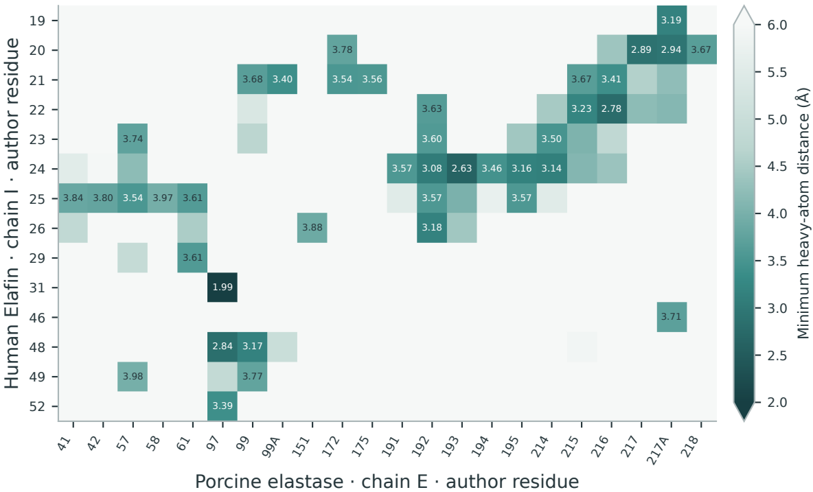
c Interface contact map (<4 Å residue set)
