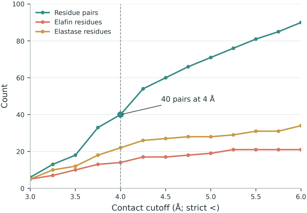
d Cutoff sensitivity of interface size
