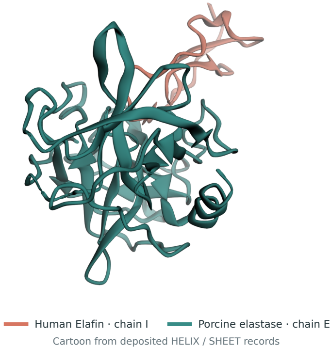
a Experimental reference complex
