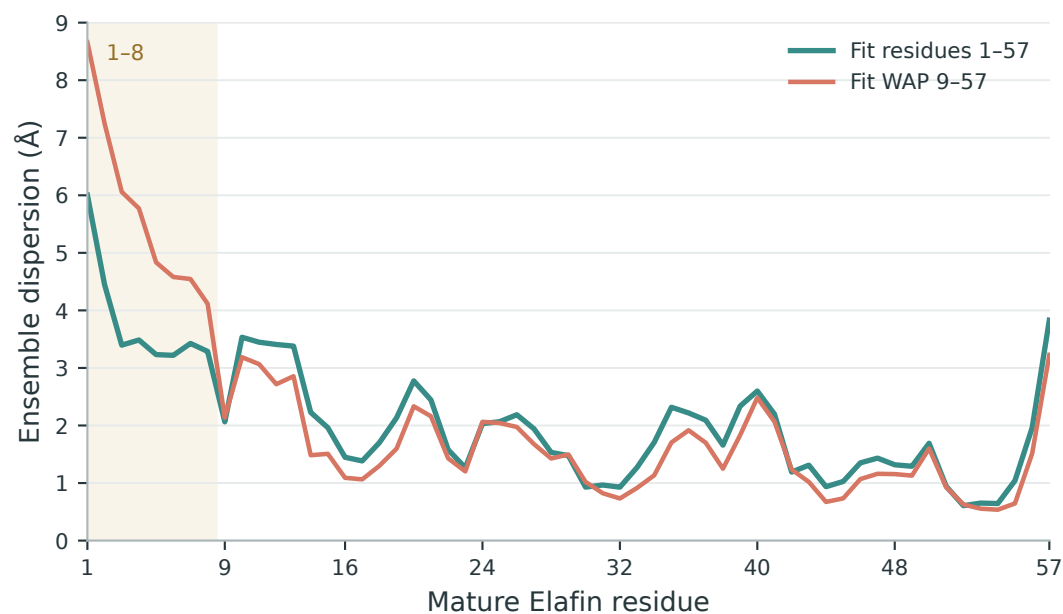
c Residue-wise spread around the aligned mean
