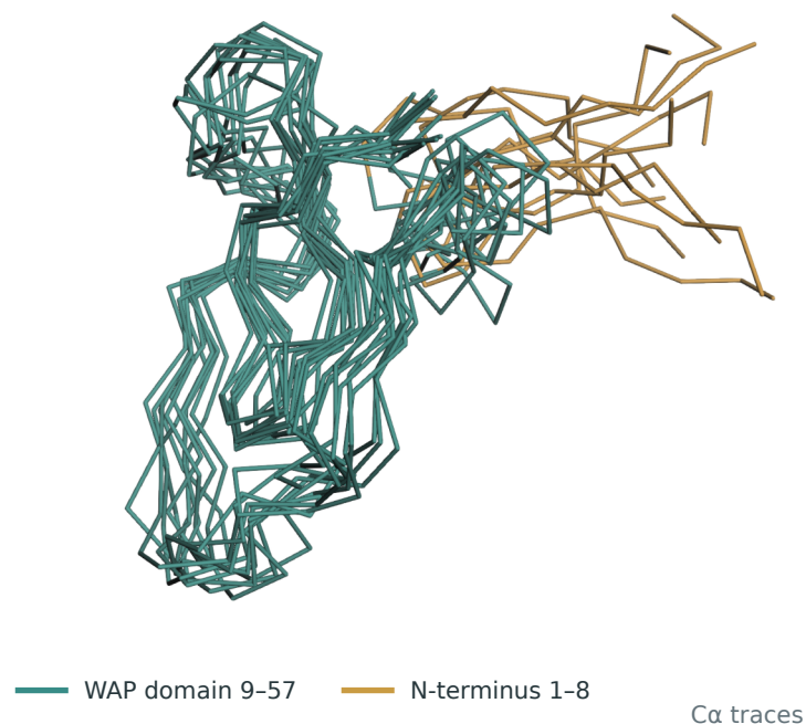
a Eleven conformers after WAP-domain alignment
