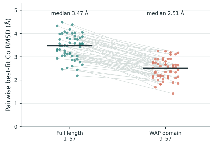
d Sensitivity to the fitted residue set
