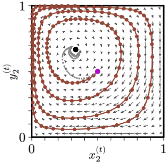
MWU ( \eta = 0.25 )
