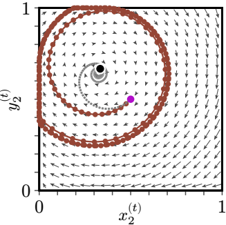
OGD ( \eta = 0.1 )
