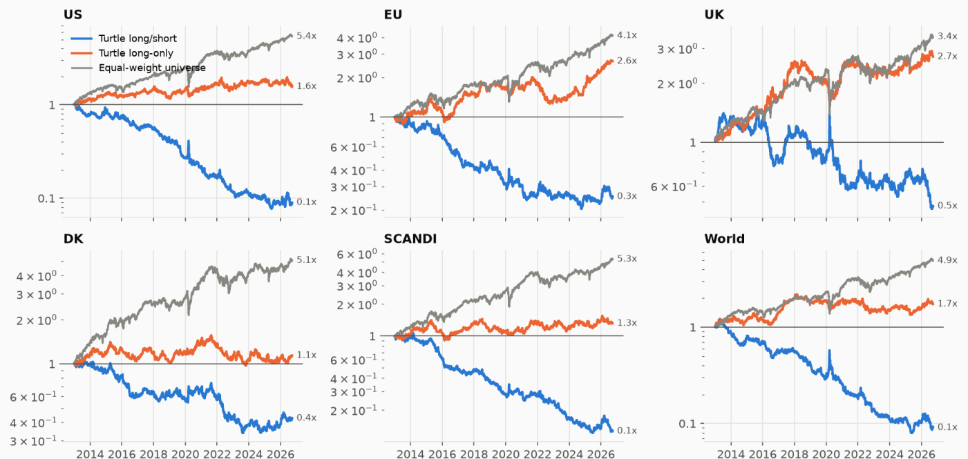
Turtle rules on six stock universes, 2013-2026
