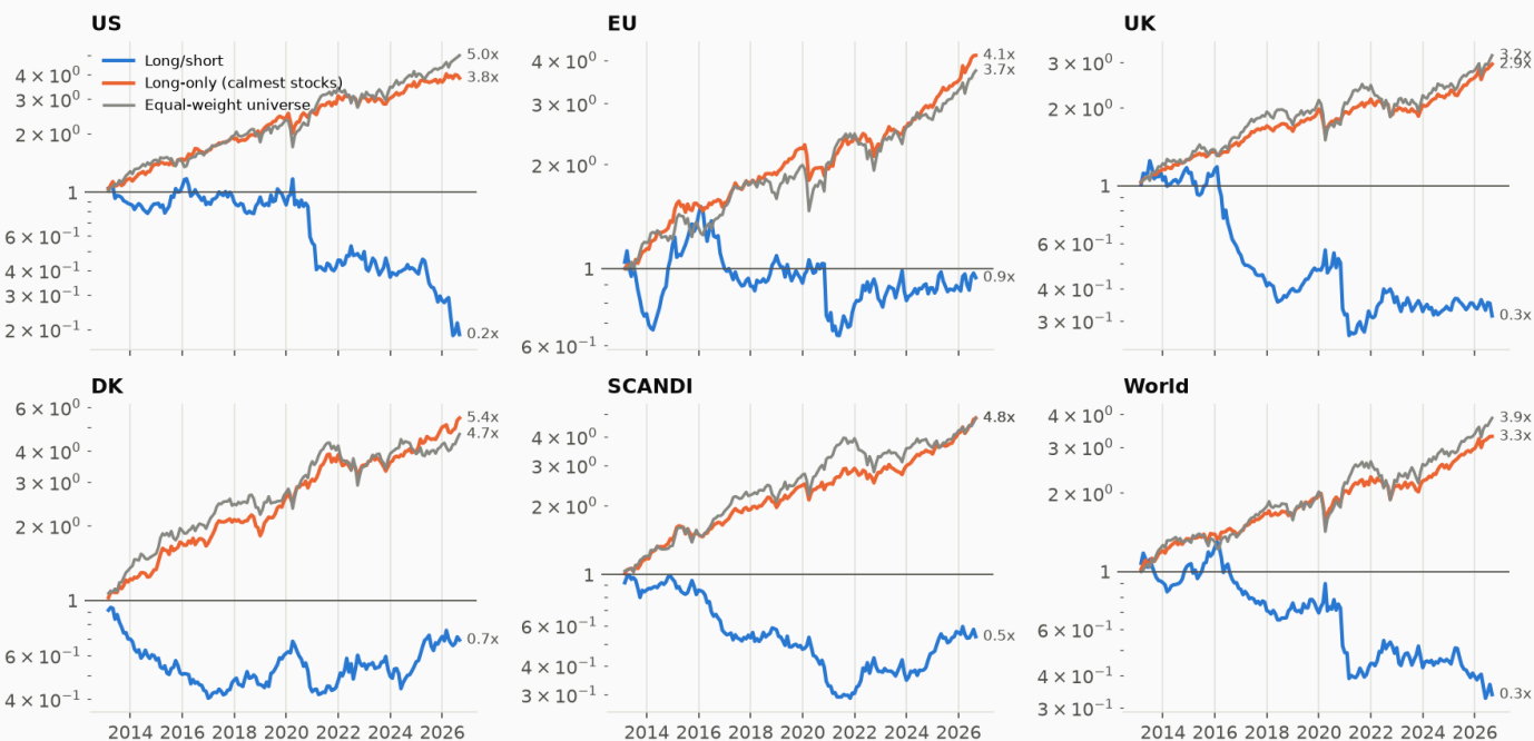
Low volatility on six stock universes, 2013-2026
