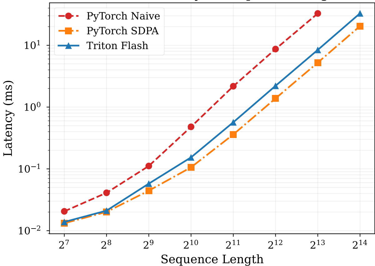
Attention Latency vs Sequence Length
